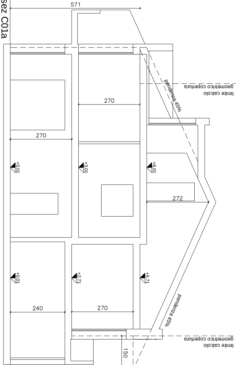
PIANO TERRA
